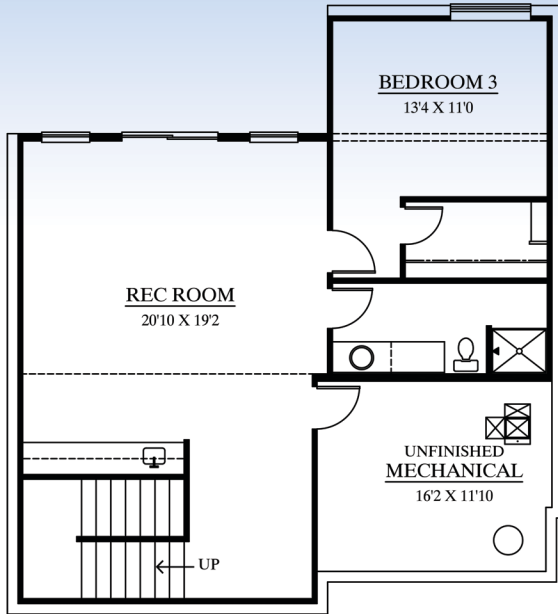
LOWER LEVEL 836 sq ft FINISHED 172 sq ft UNFINISHED
