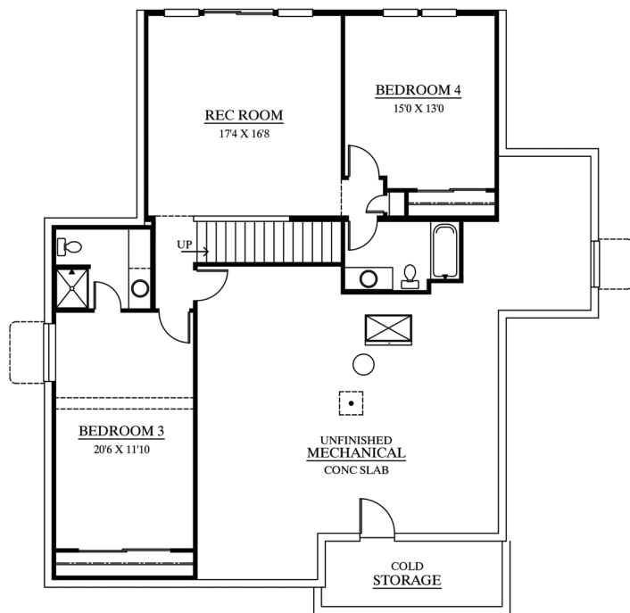
LOWER LEVEL 1028 sq ft FINISHED 742 sq ft UNFINISHED 88 sq ft COLD STORAGE
