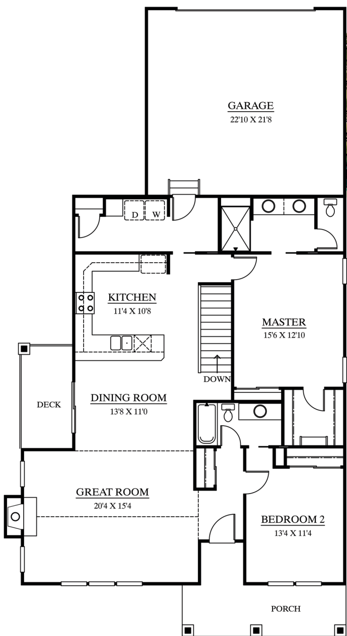
MAIN LEVEL 1532 sq ft FINISHED 518 sq ft GARAGE
