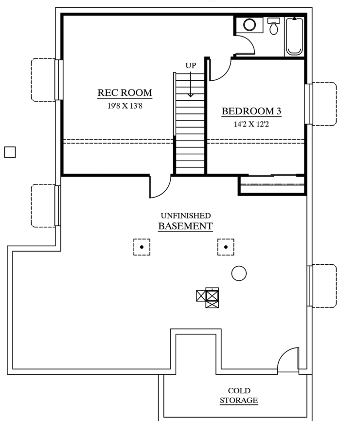
LOWER LEVEL 646 sq ft FINISHED 778 sq ft UNFINISHED 120 sq ft COLD STORAGE
